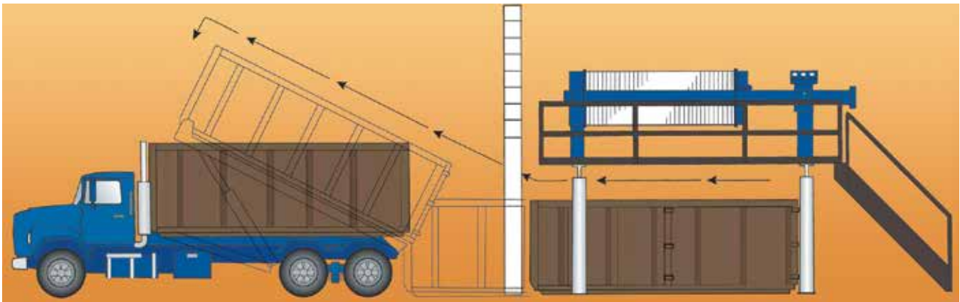
Self-dumping dumpsters
